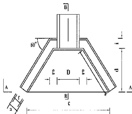
CULVERT TYPES
