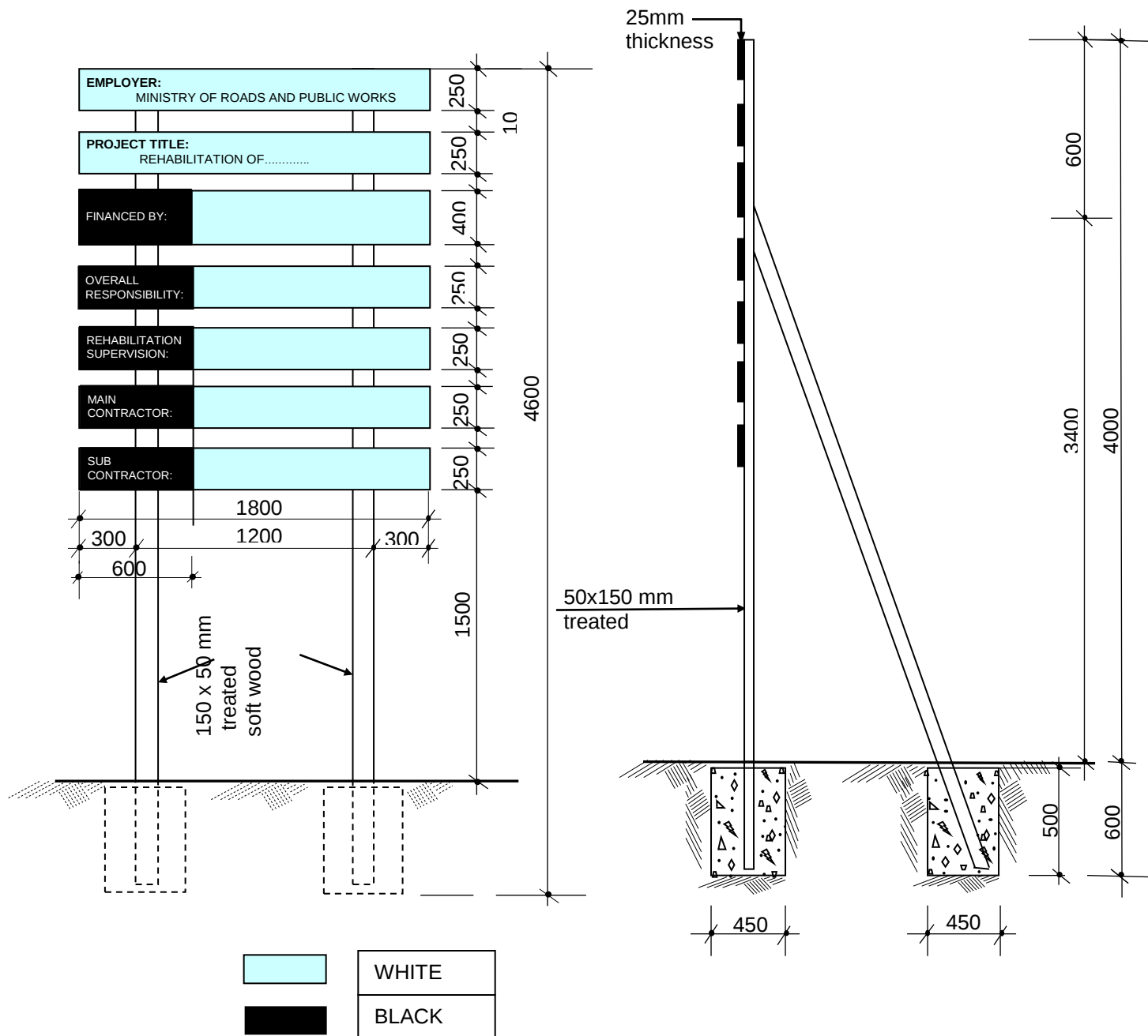
FIGURE C.17 - PUBLICITY SIGNBOARD
