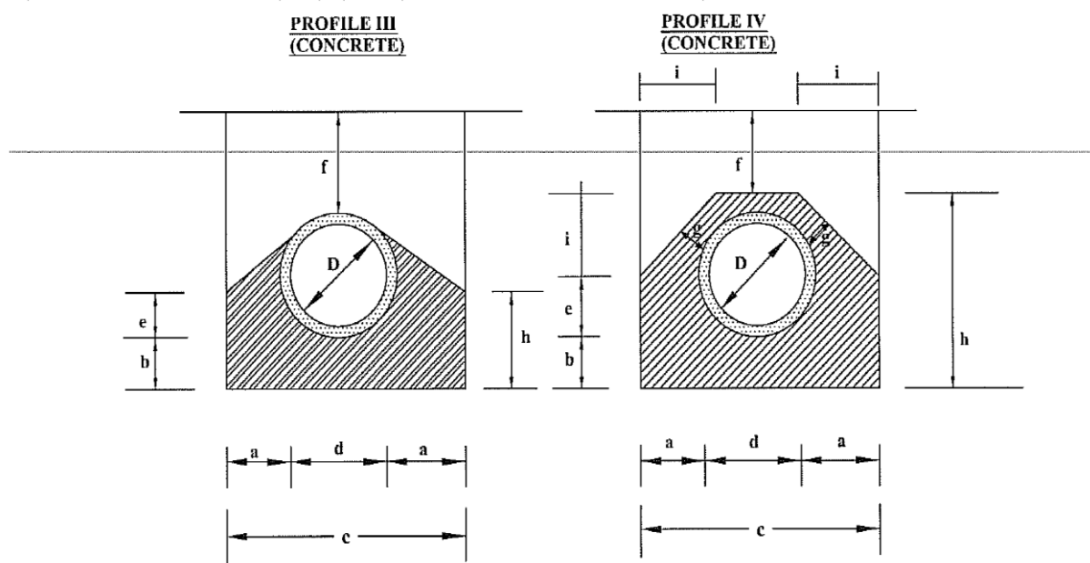
FIGURE C17-BEDDING AND SURROUND PROFILE TYPES III &amp; IV
