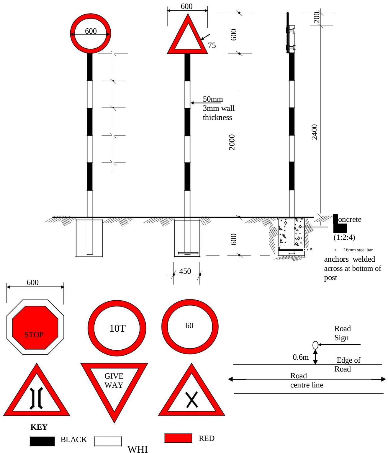
FIGURE C.16 - TRAFFIC SIGNS
