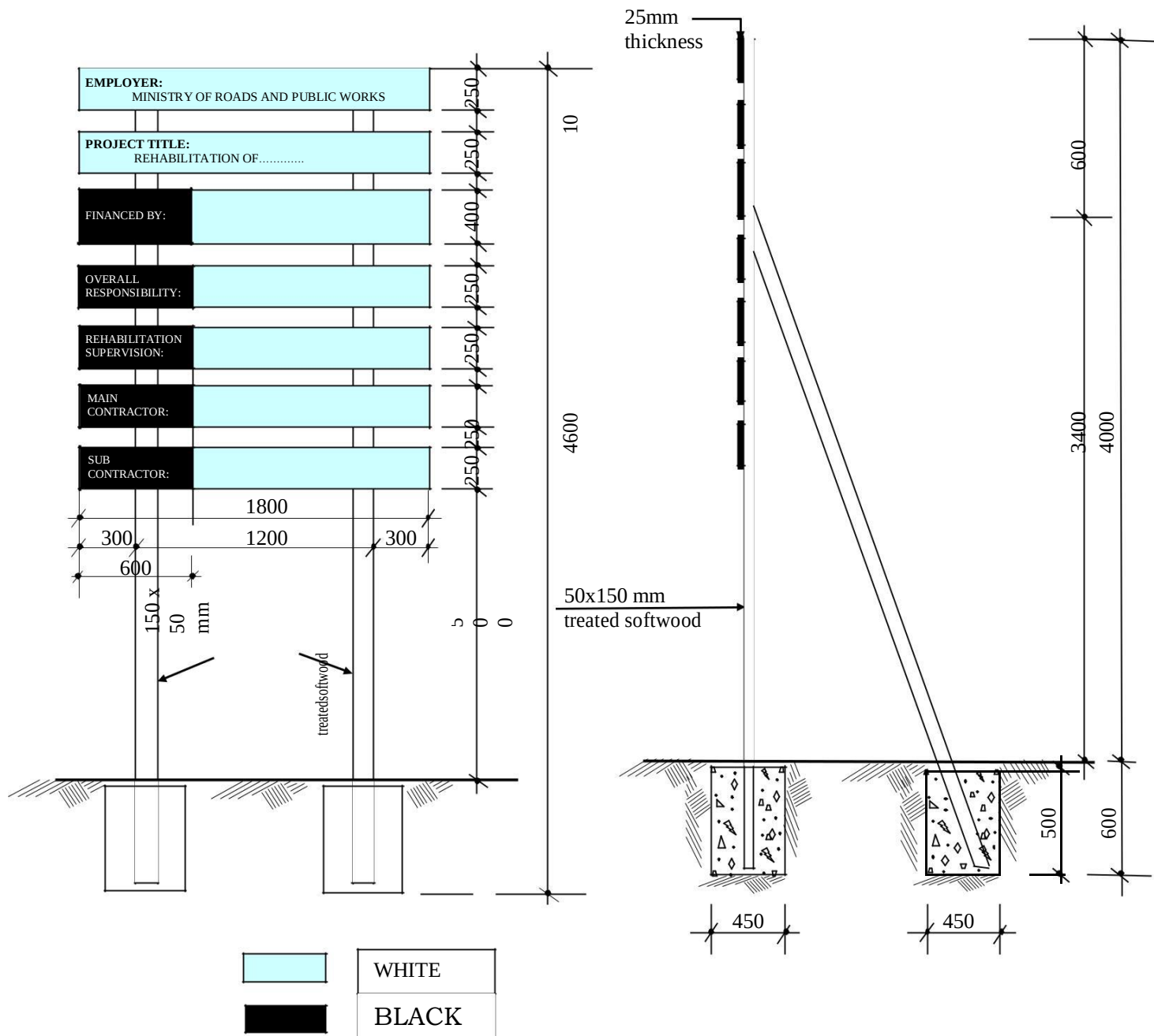
FIGURE C.17 - PUBLICITY SIGNBOARD
