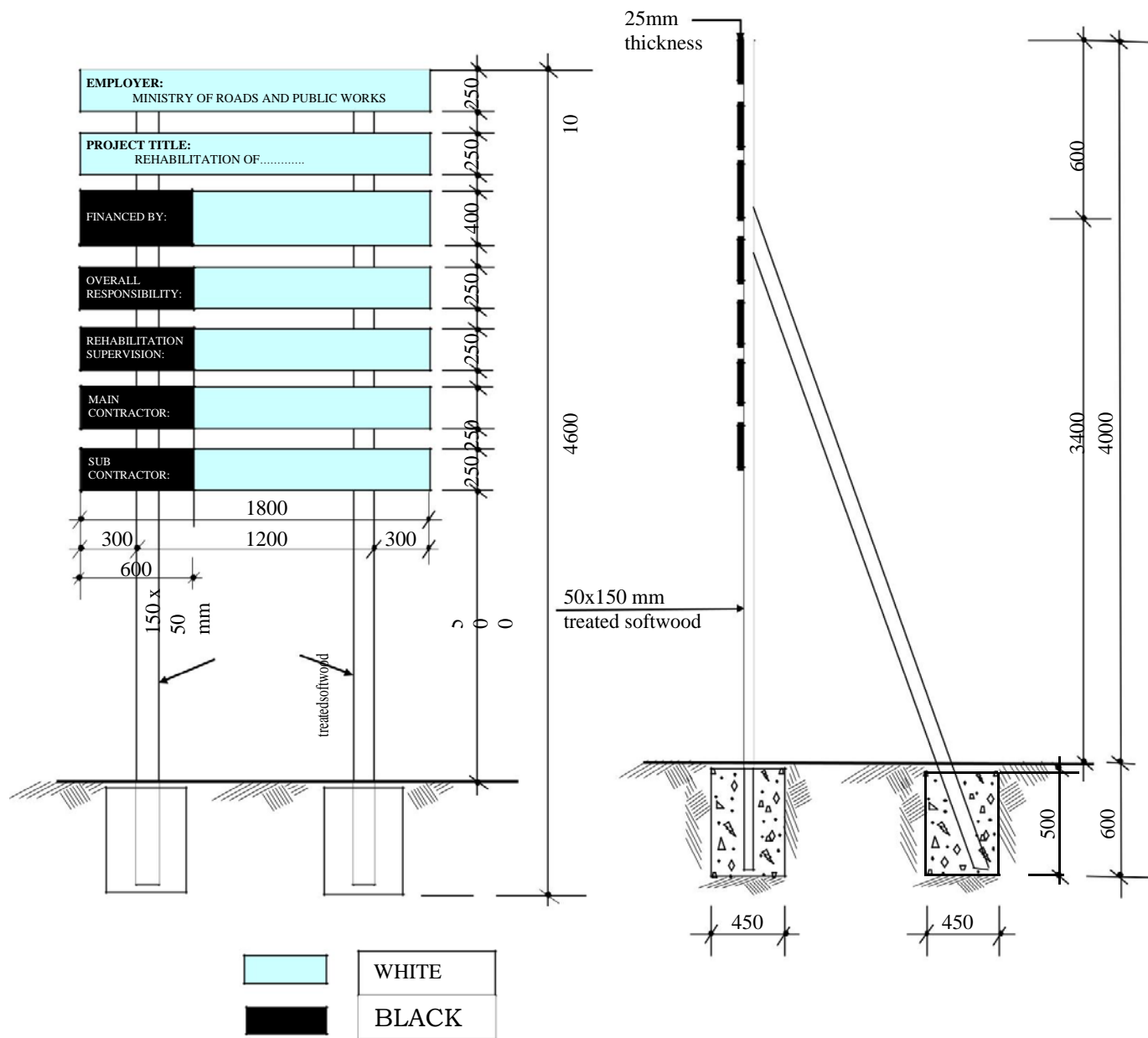
FIGURE C.17 - PUBLICITY SIGNBOARD
