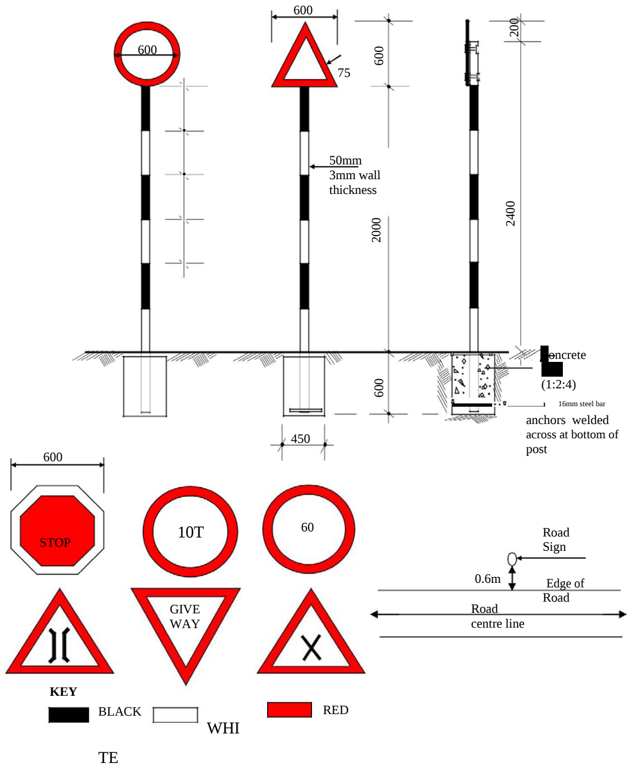
FIGURE C.16 - TRAFFIC SIGNS
