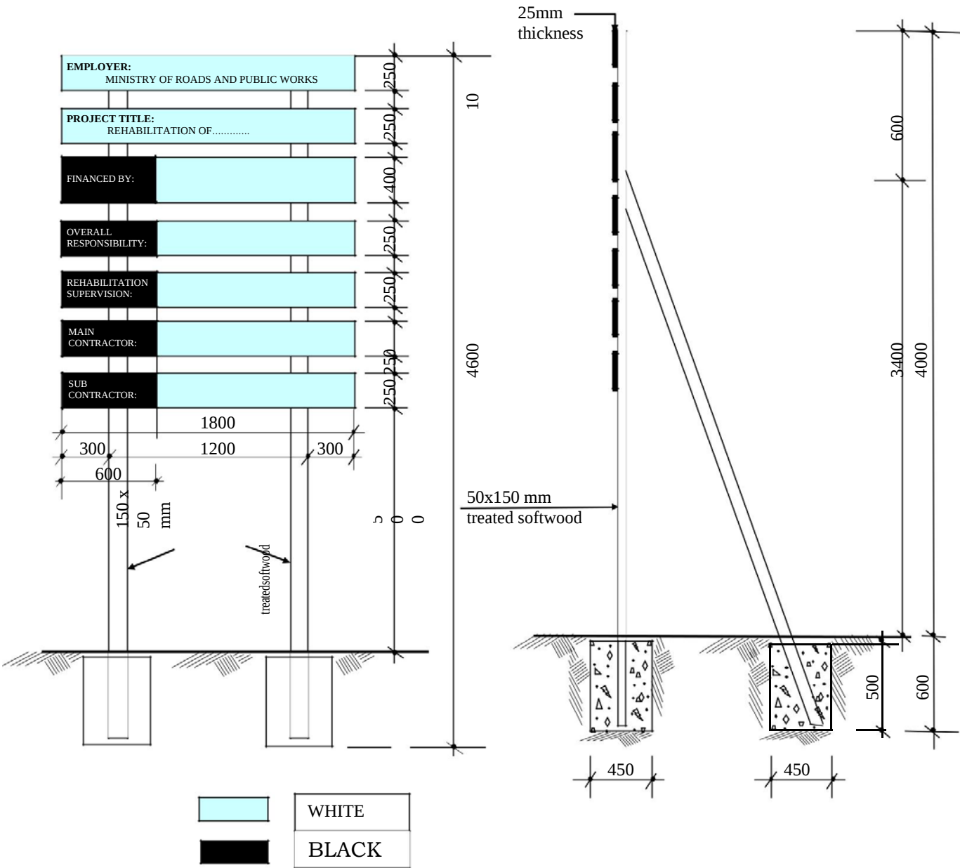
FIGURE C.17 - PUBLICITY SIGNBOARD
