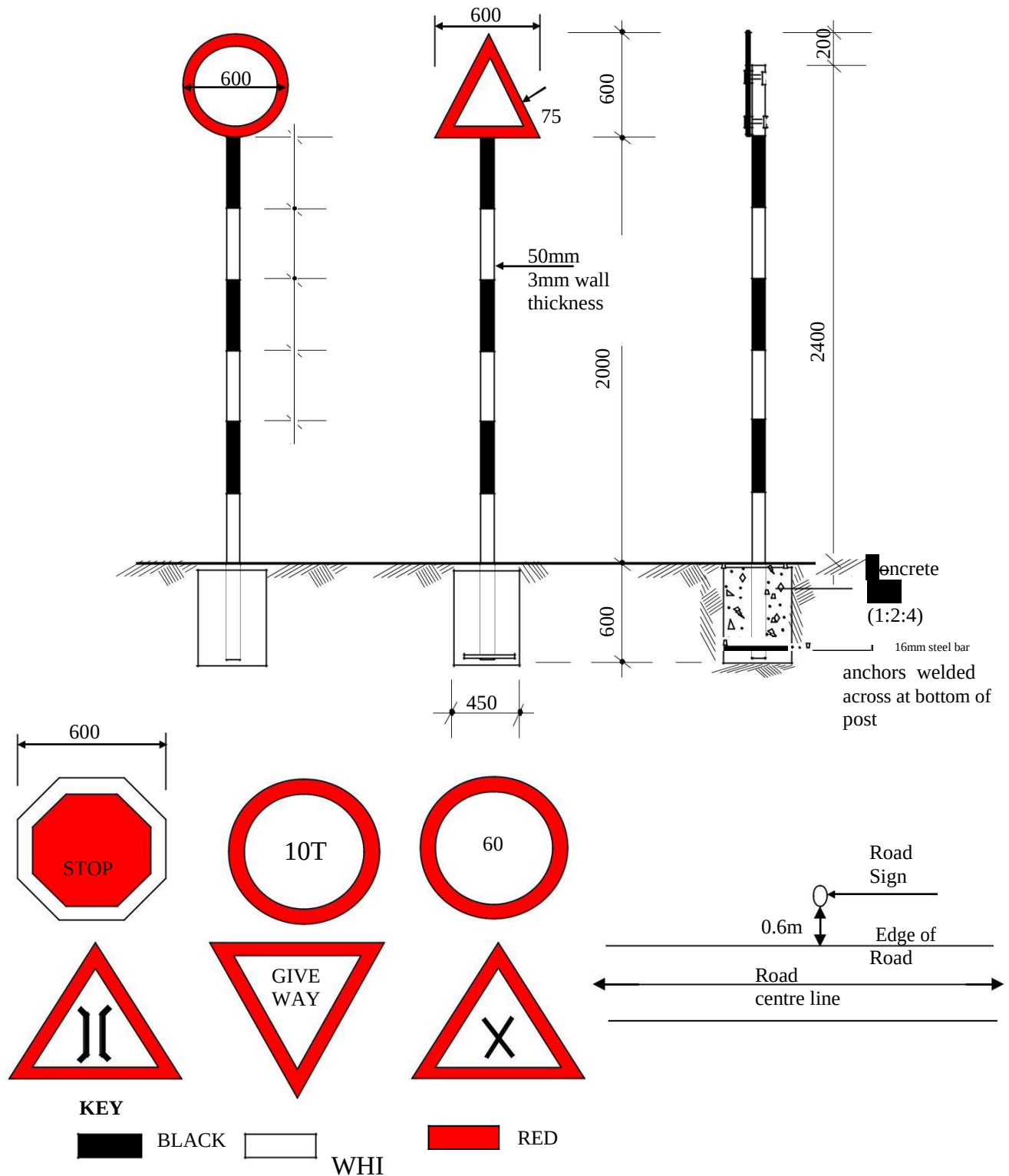
FIGURE C.16 - TRAFFIC SIGNS
