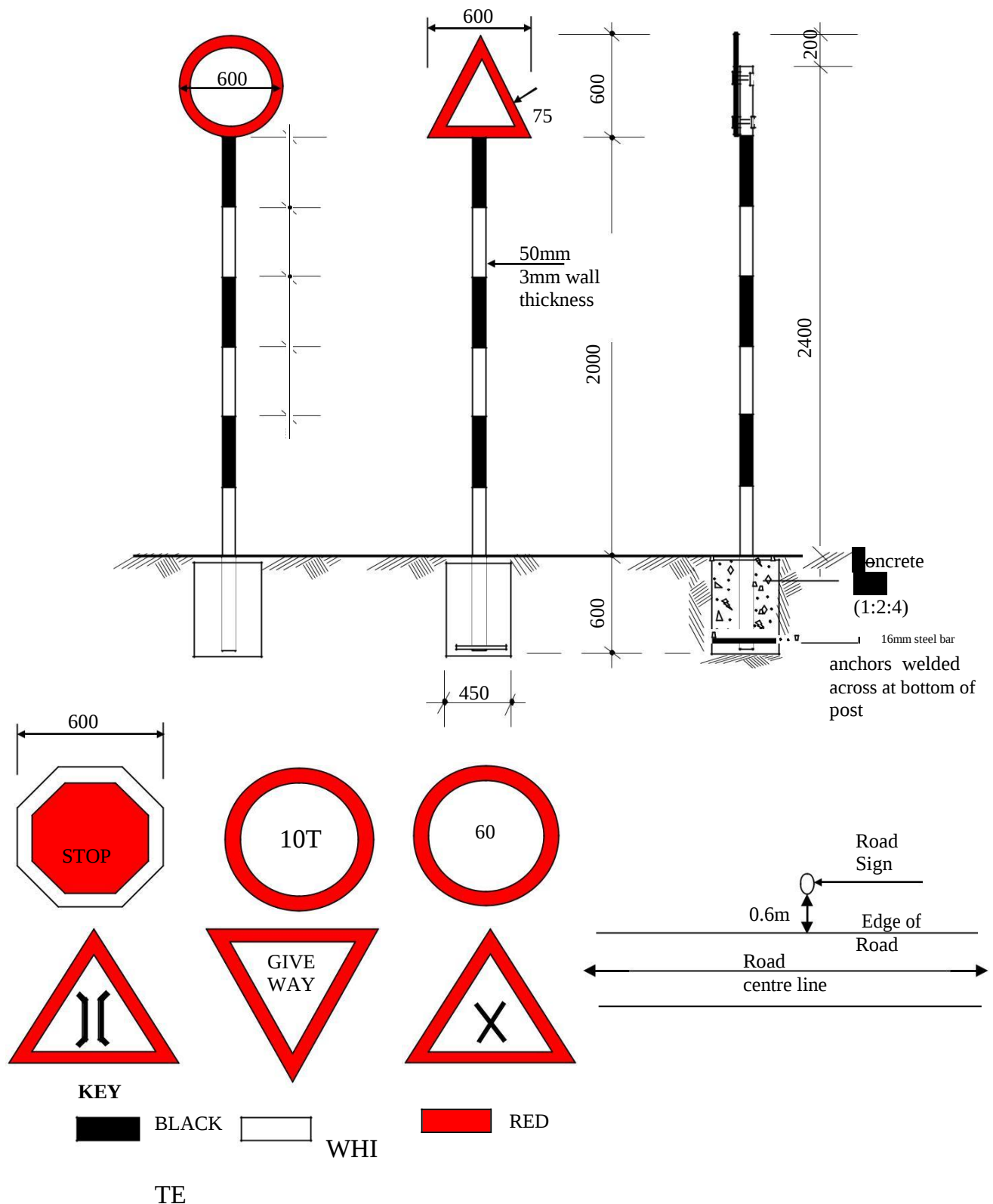
FIGURE C.16 - TRAFFIC SIGNS
