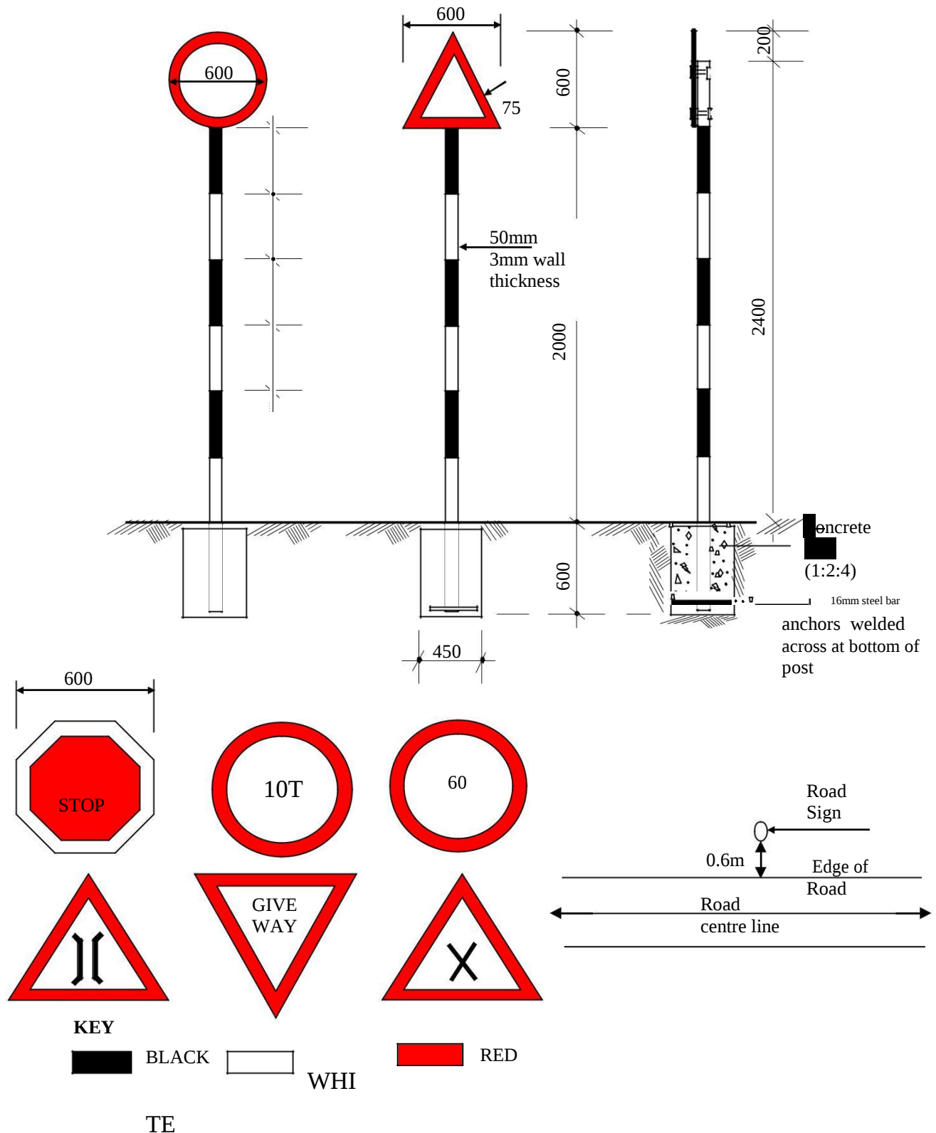
FIGURE C.16 - TRAFFIC SIGNS
