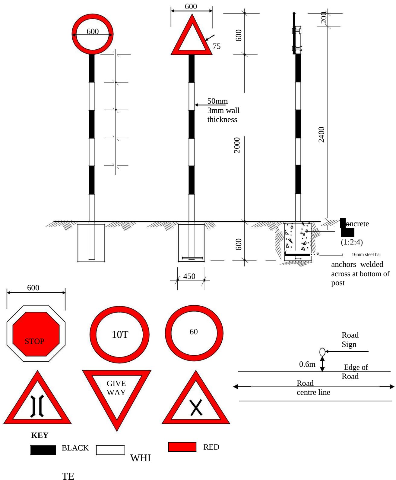
FIGURE C.16 - TRAFFIC SIGNS
