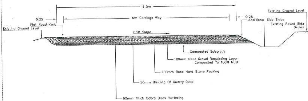
TYPICAL CROSS SECTION: TYPE 1
