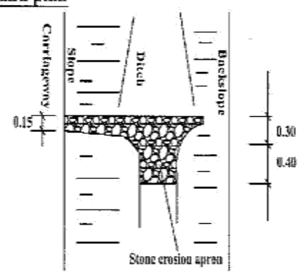
Ground plan
